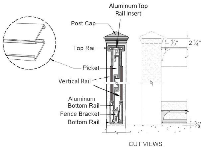
CUT VIEWS
