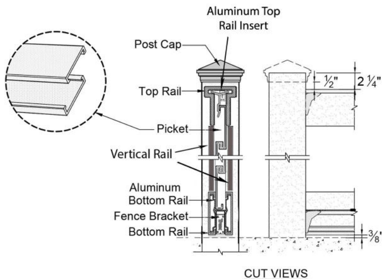
CUT VIEWS
