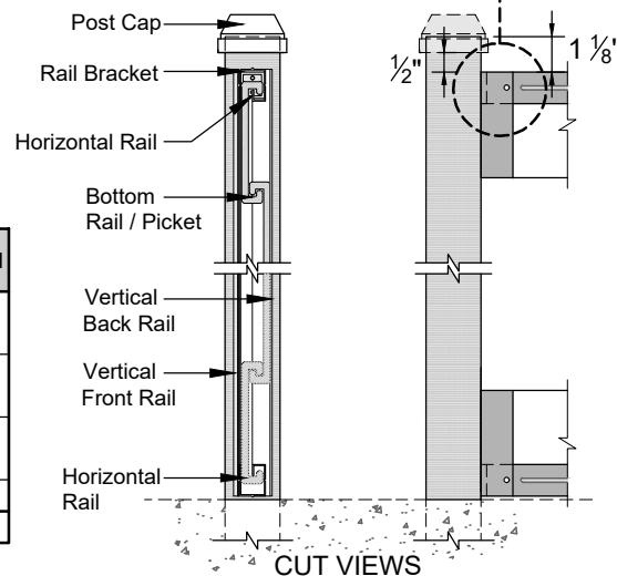
CUT VIEWS
