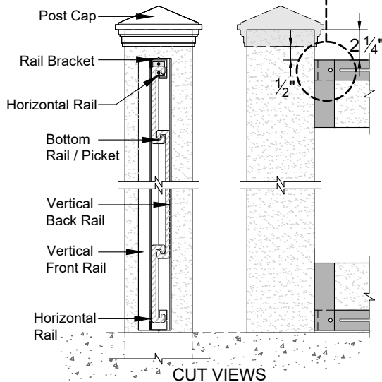
CUT VIEWS
