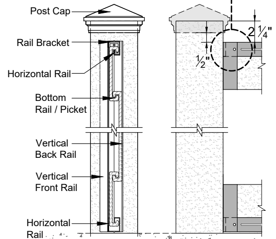
CUT VIEWS
