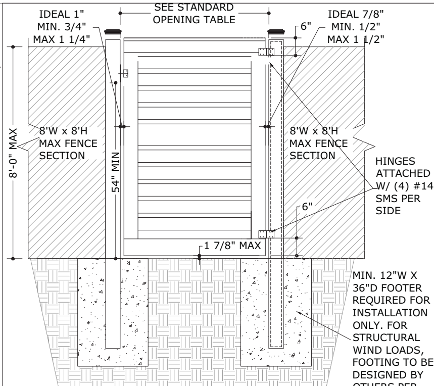
2 COMPOSITE SINGLE GATE 1 SCALE: NTS ELEVATION VIEW
