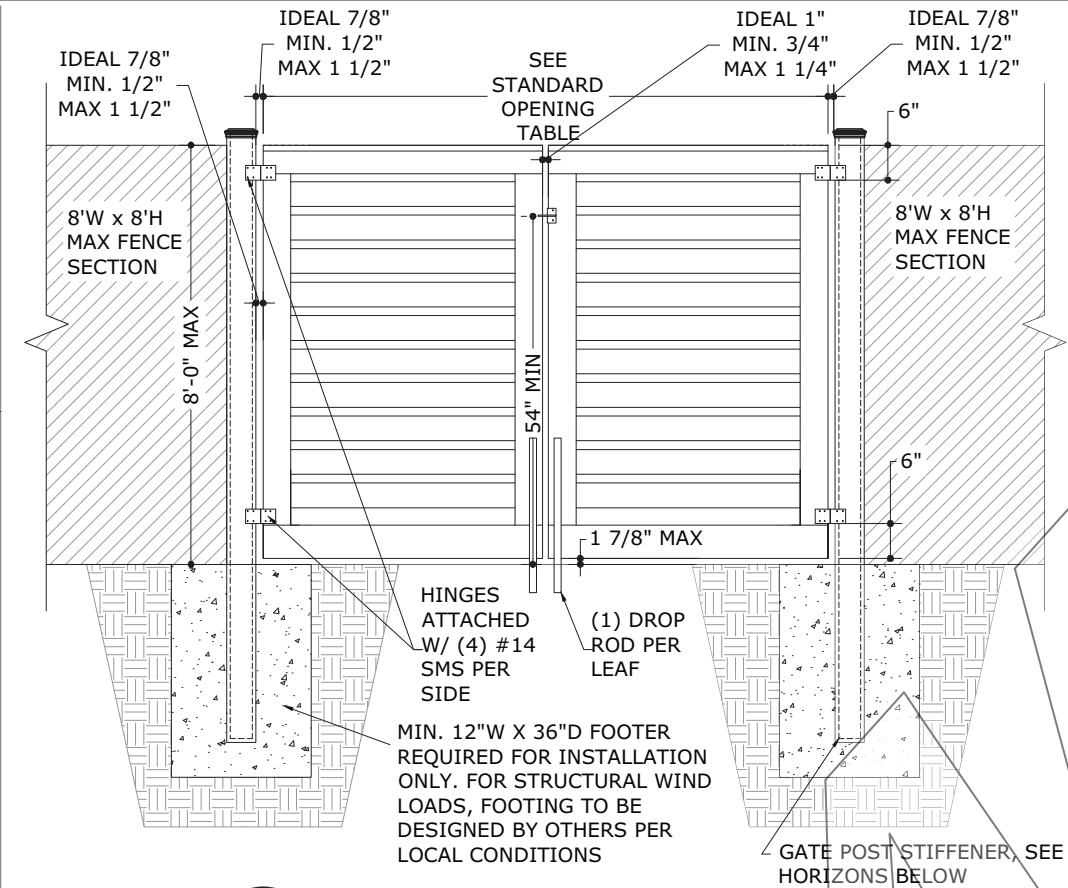
1 COMPOSITE DOUBLE GATE 1 SCALE: NTS ELEVATION VIEW
