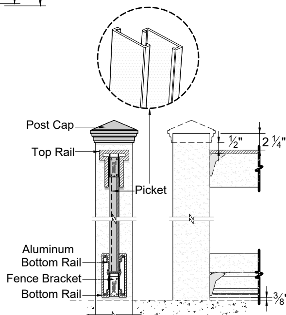
CUT VIEWS
